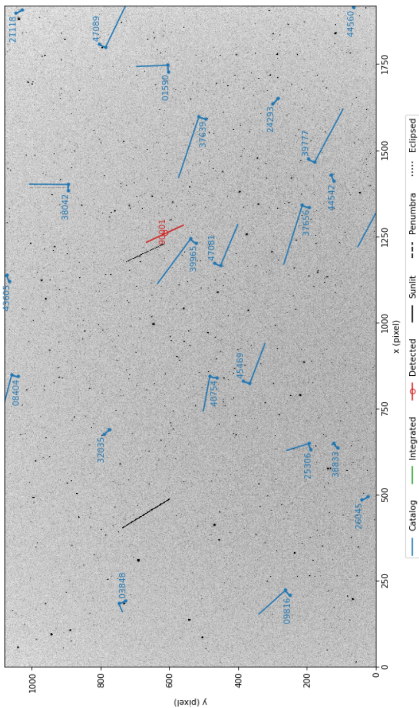
Figure 9.5: stvid processed image, with three unidentified satellites, the second labeled with NORAD ID 90001.
