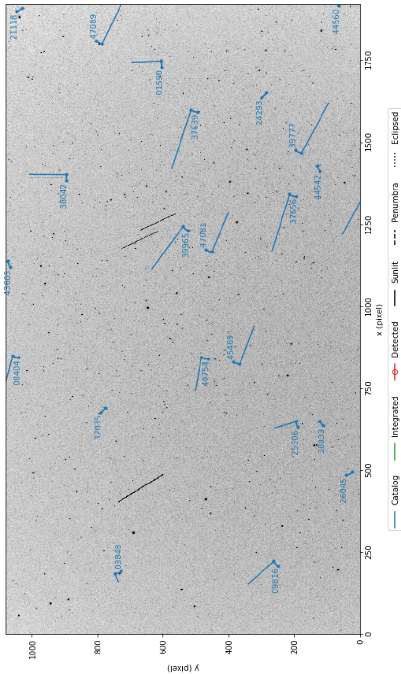
Figure 9.3: stvid processed image, with three unidentified satellites.
