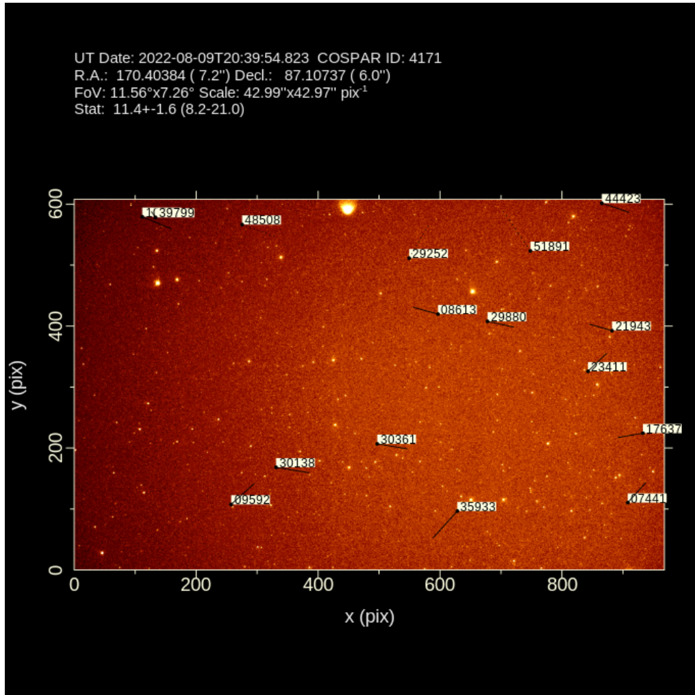
Figure 9.1: satid example.
