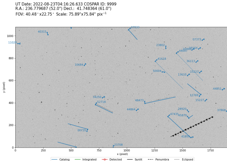
Figure 10.1: stvid PNG.
