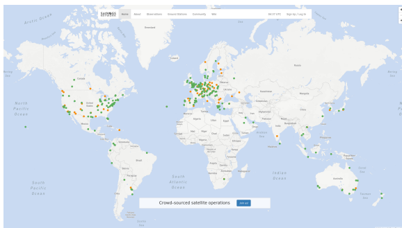
Figure 1: SatNOGS Network.
