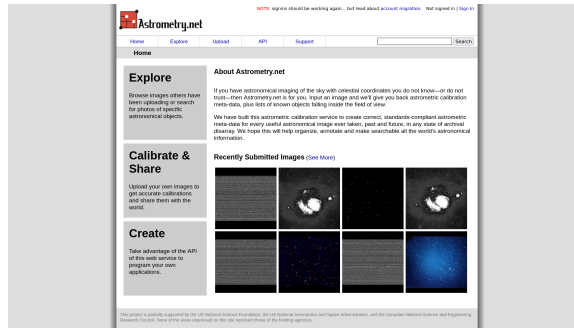
Figure 7.1: nova.astrometry.net website.
